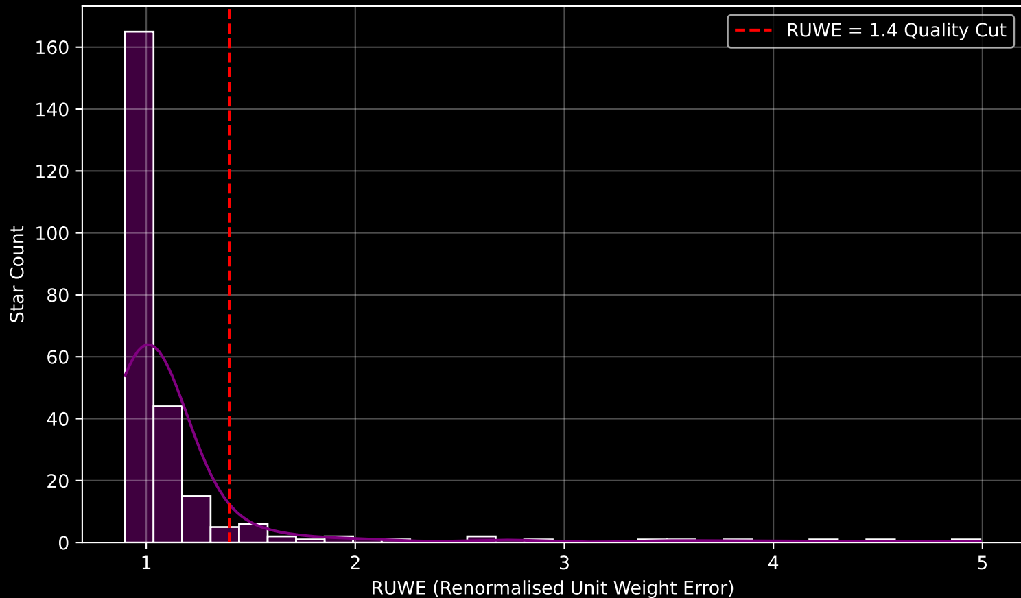
GALAH DR4 Field [350] RUWE Distribution (n= 251)
