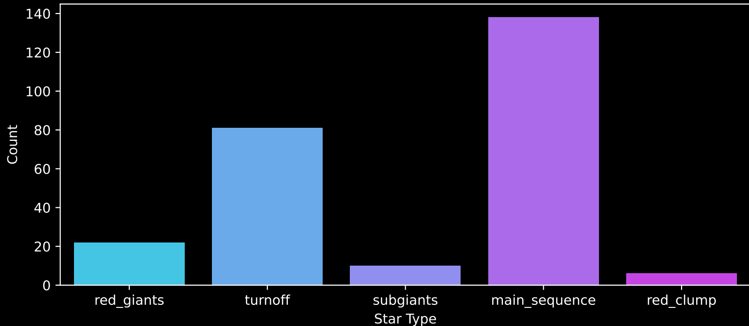
GALAH DR4 Field: [350] Count plot of Star Type
